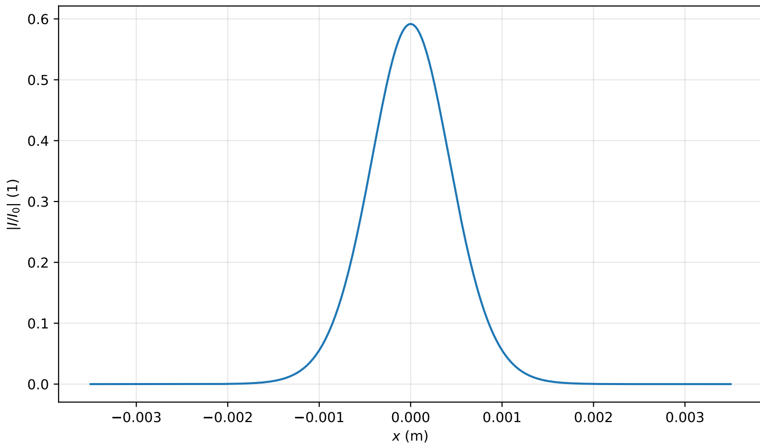
Intensity profile I(x, y = 0, z = 2.229m)/I_0 , P_{in}=0.3P_{cr} , artificial time
